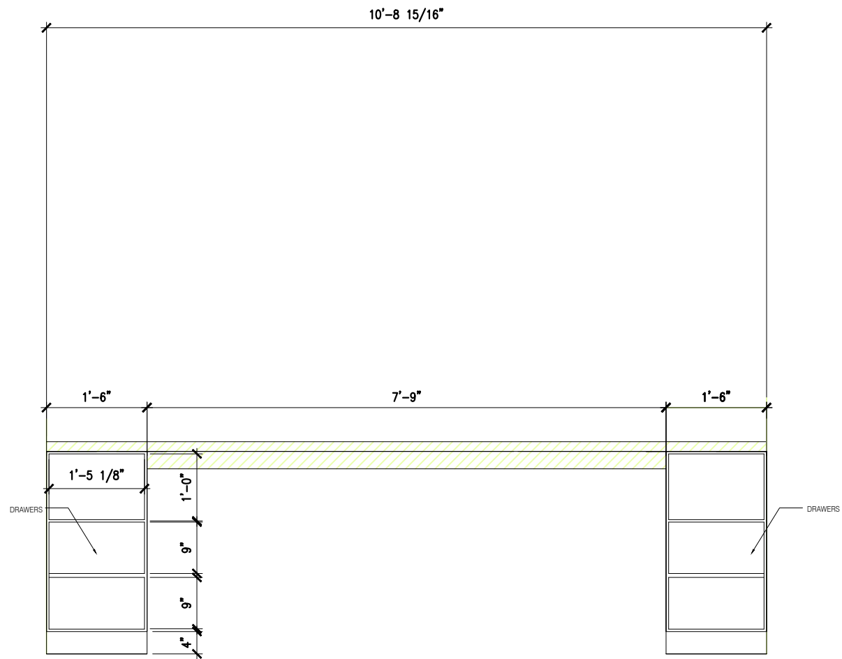
SIDE VIEW 2
